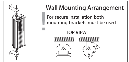
ASC-40T 30W/100V
